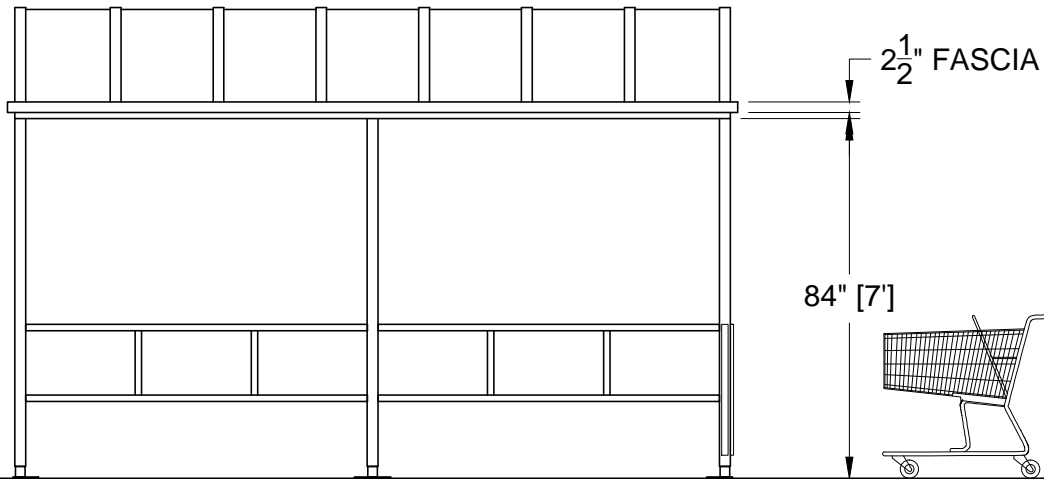
SIDE ELEVATION
